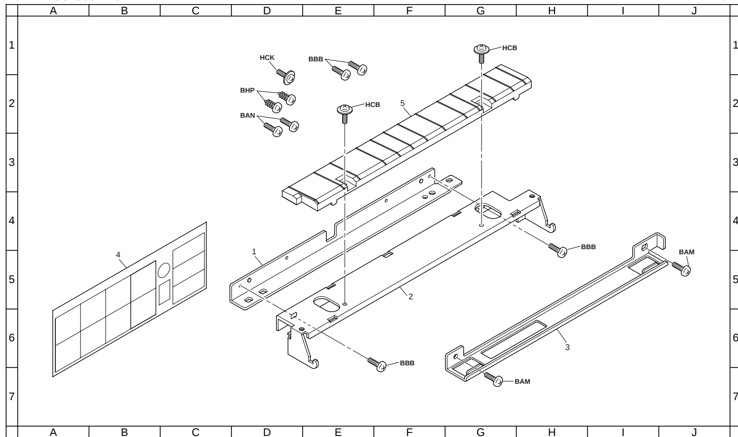
FIG. 4 ACCESSORIES
